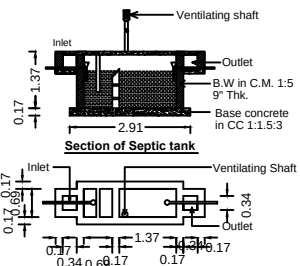
SEPTIC TANK DETAIL
