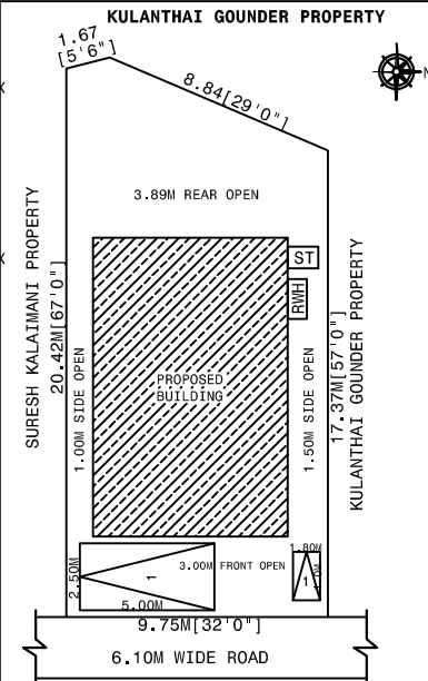
SITE PLAN SCALE:1"=16'0" [1:200]
