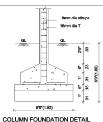
COLUMN FOUNDATION DETAIL
