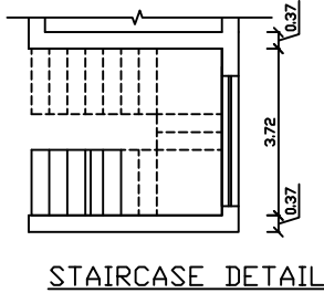
STAIRCASE DETAIL
