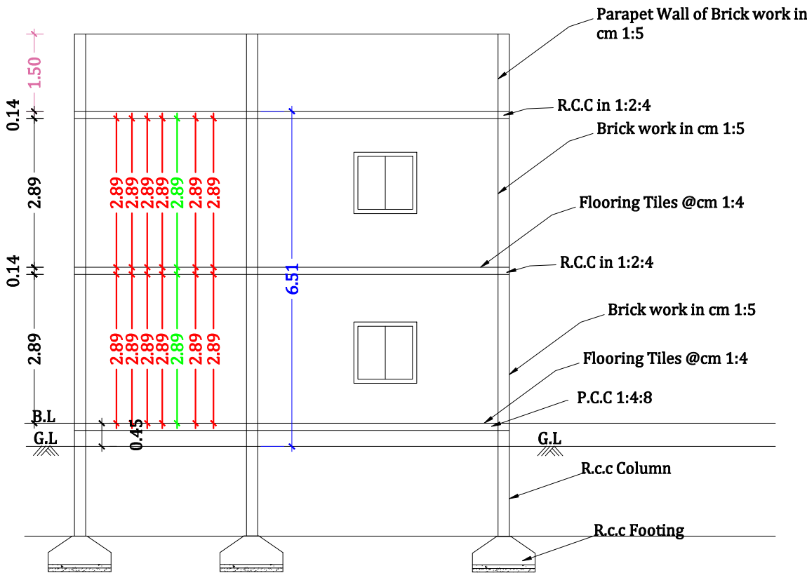
SECTION IN AA SCALE 1:100
