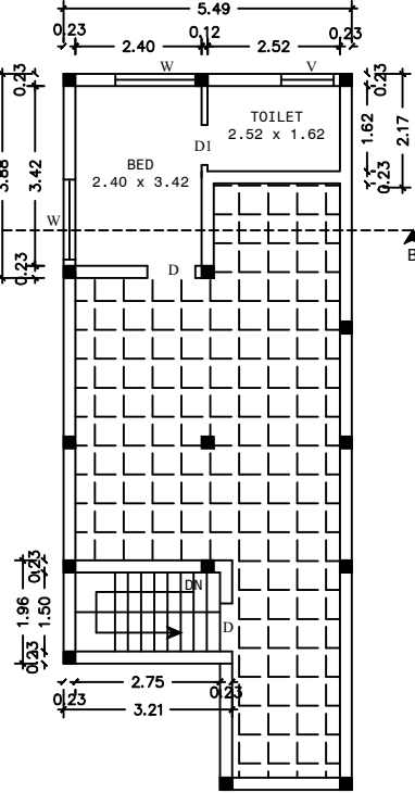
FIRST FLOOR PLAN (SCALE 1:100)
