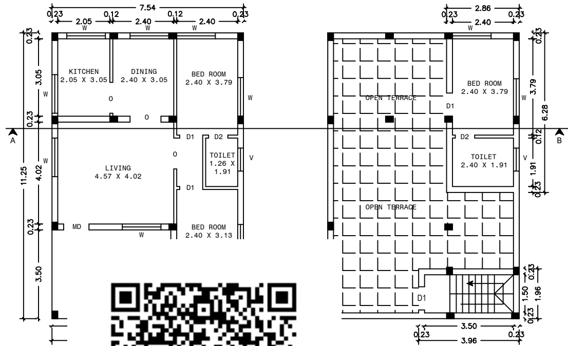
FIRST FLOOR PLAN (SCALE 1:100)
