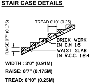
STAIR CASE DETAILS
