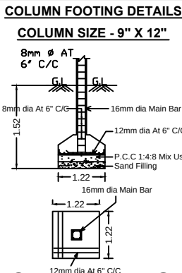
COLUMN FOOTING DETAILS
