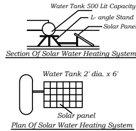
Section Of Solar Water Heating System
