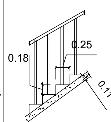
STAIRCASE DETAILS:-
