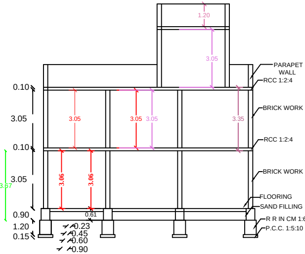
SECTION AB
