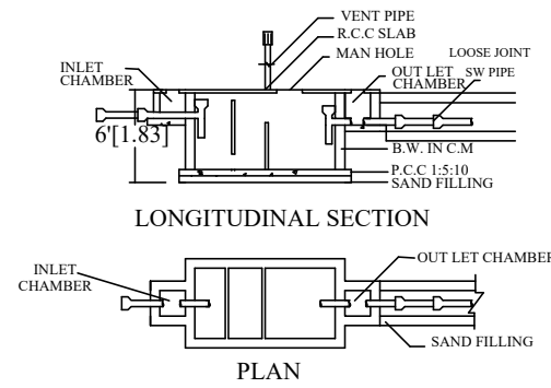
SEPTIC TANK:
