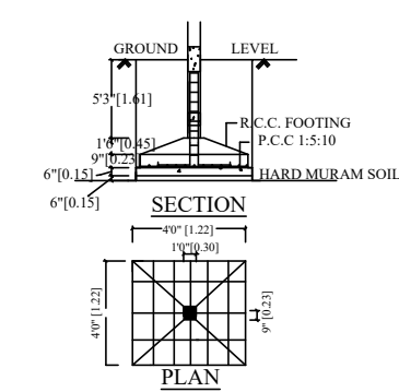
FOUNDATION DETAILS
