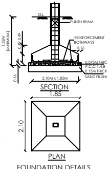
FOUNDATION DETAILS
