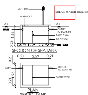
PLAN SEPTIC. TANK
