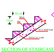
SECTION OF STAIRCASE
