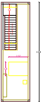
FIRST FLOOR PLAN
