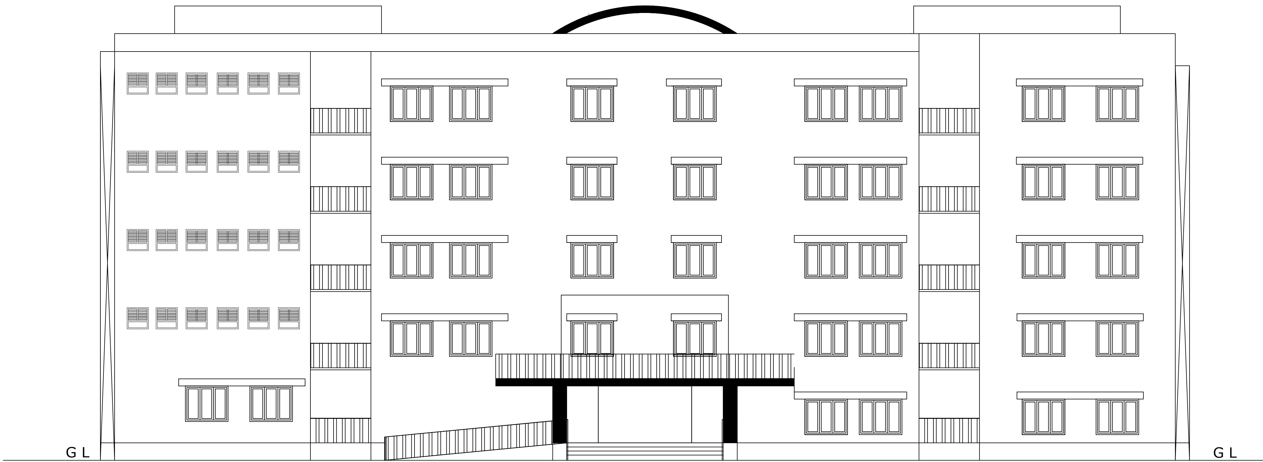
FRONT ELEVATION
