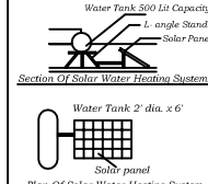
Plan Of Solar Water Heating System
