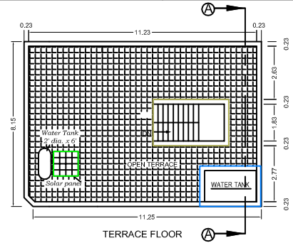
Plan Of Solar Water Heating System
