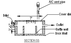
SECTION SS
