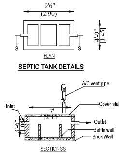
SECTION SS
