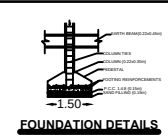
FOUNDATION DETAILS
