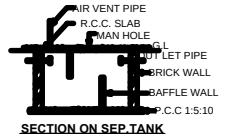
SECTION ON SEP. TANK
