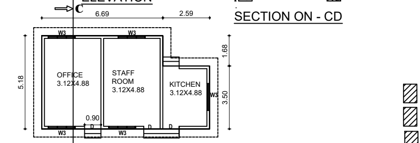
OFFICE, STAFF ROOM KITCHEN - PLAN
