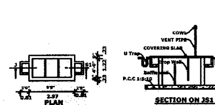
SECTION ON 'J51'
