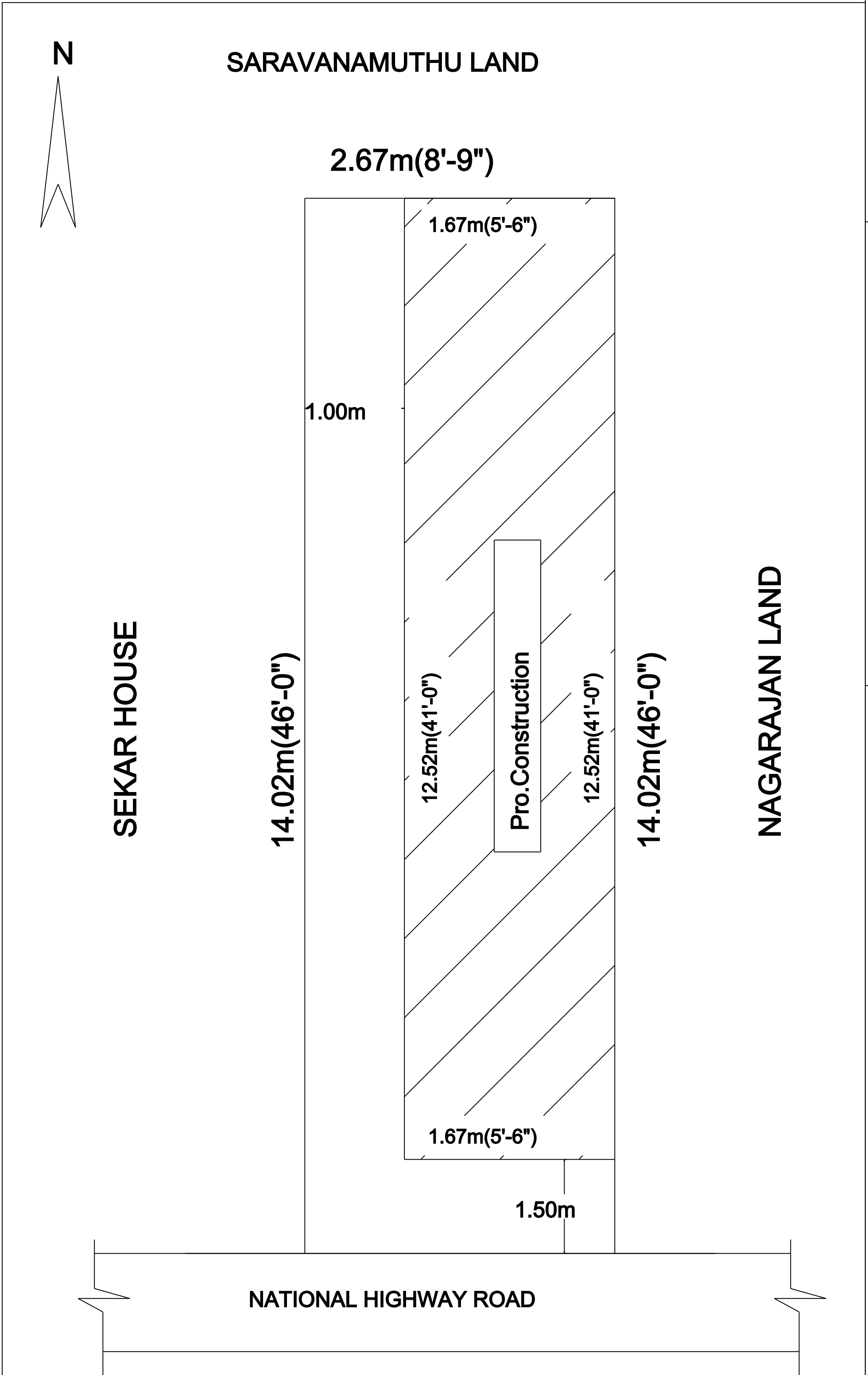
SITE PLAN
