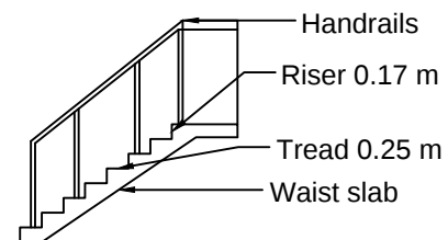
STAIRCASE DETAILS
