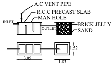
DETAILS OF SEPTIC TANK & DISPERSION TRENCH
