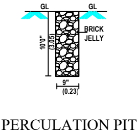
PERCULATION PIT
