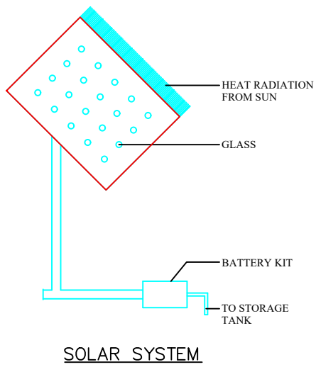
SOLAR SYSTEM
