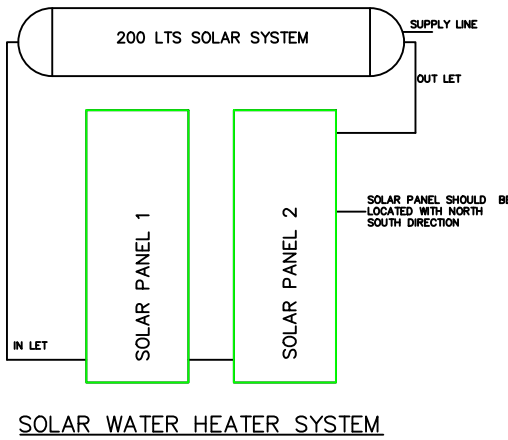
SOLAR WATER HEATER SYSTEM
