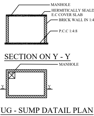
UG - SUMP DETAIL PLAN
