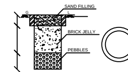
RAIN WATER HARVESTING SYSTEM
