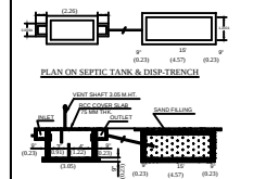
SECTION ON SEPTIC TANK & DISP-TRENCH
