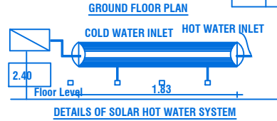
DETAILS OF SOLAR HOT WATER SYSTEM
