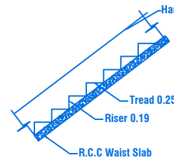
STAIR DETAILS
