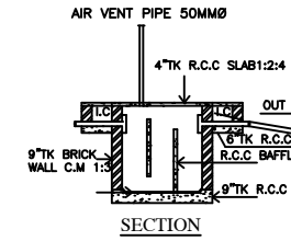
SECTION
