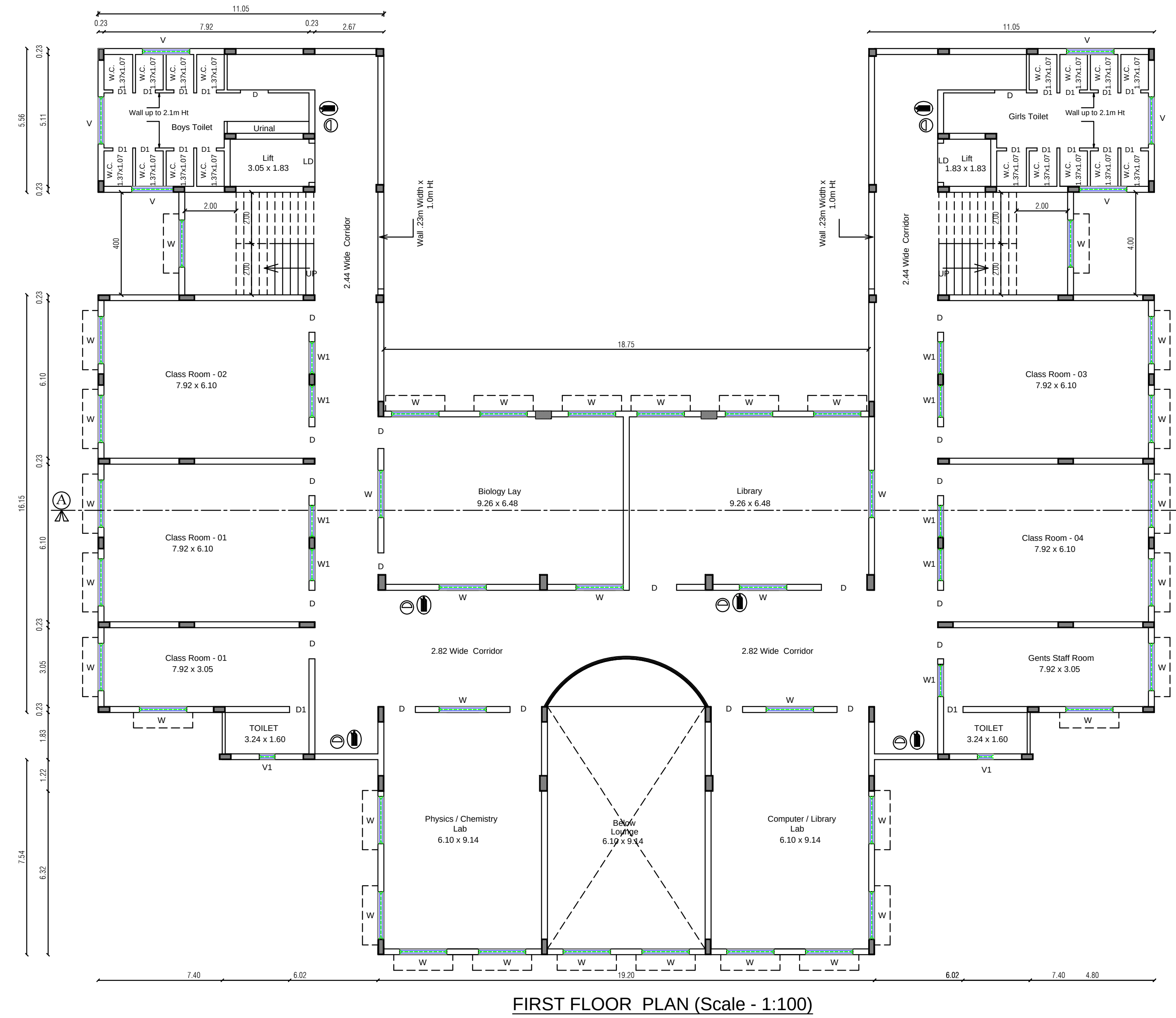
FIRST FLOOR PLAN (Scale - 1:100)
