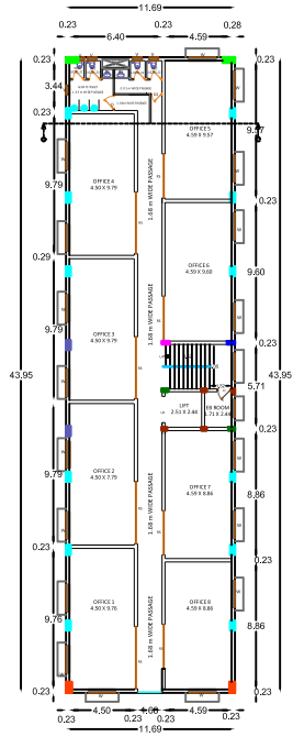
TYPICAL 2,4 FLOOR PLAN
