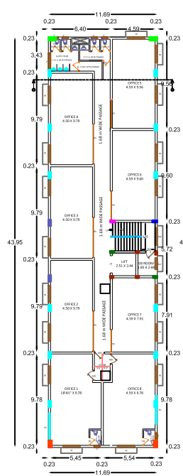
THIRD FLOOR PLAN
