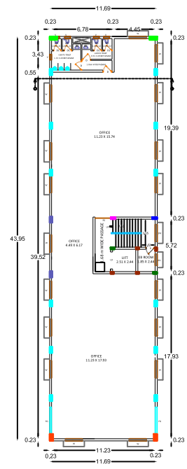
FIFTH FLOOR PLAN
