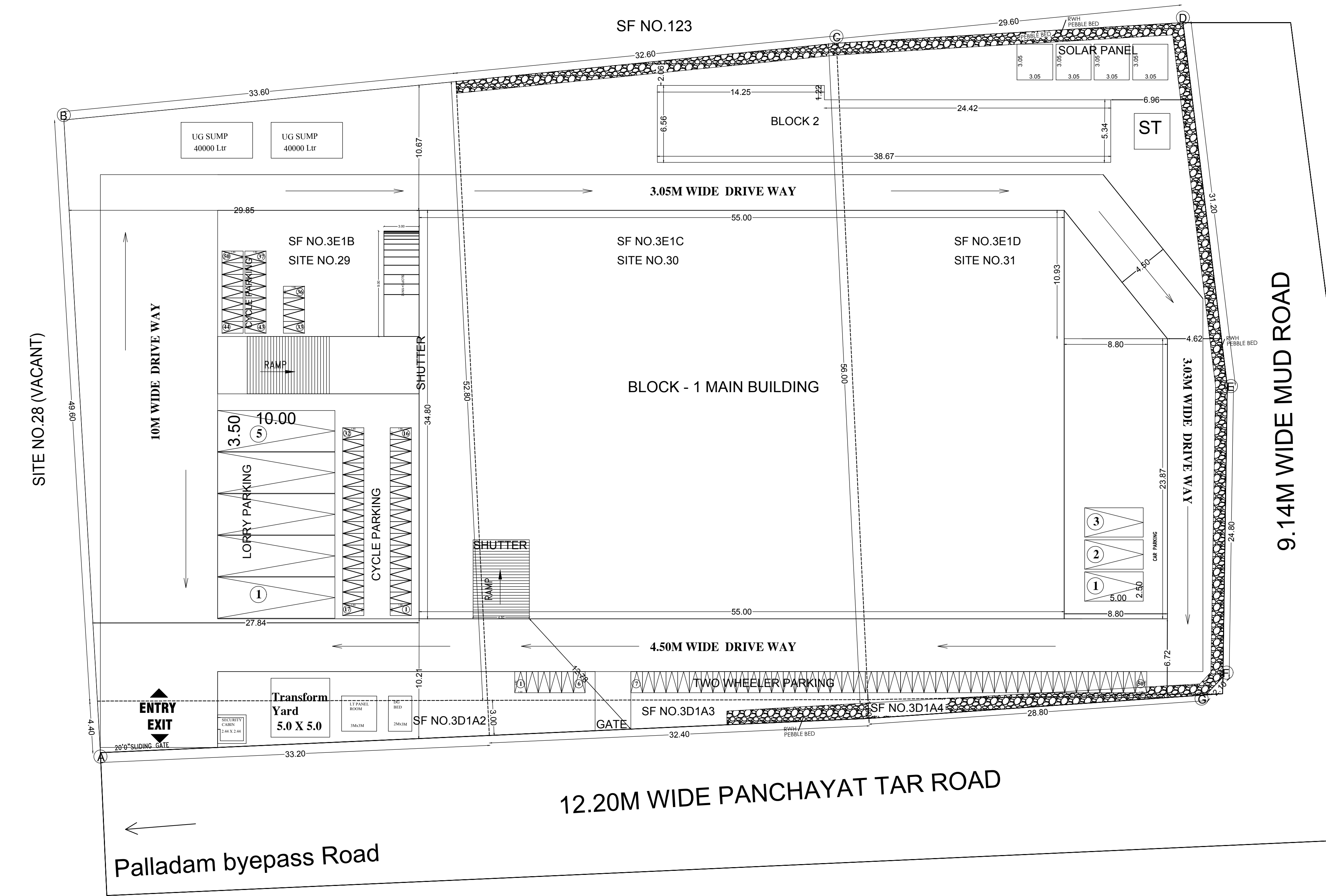
SITE PLAN
