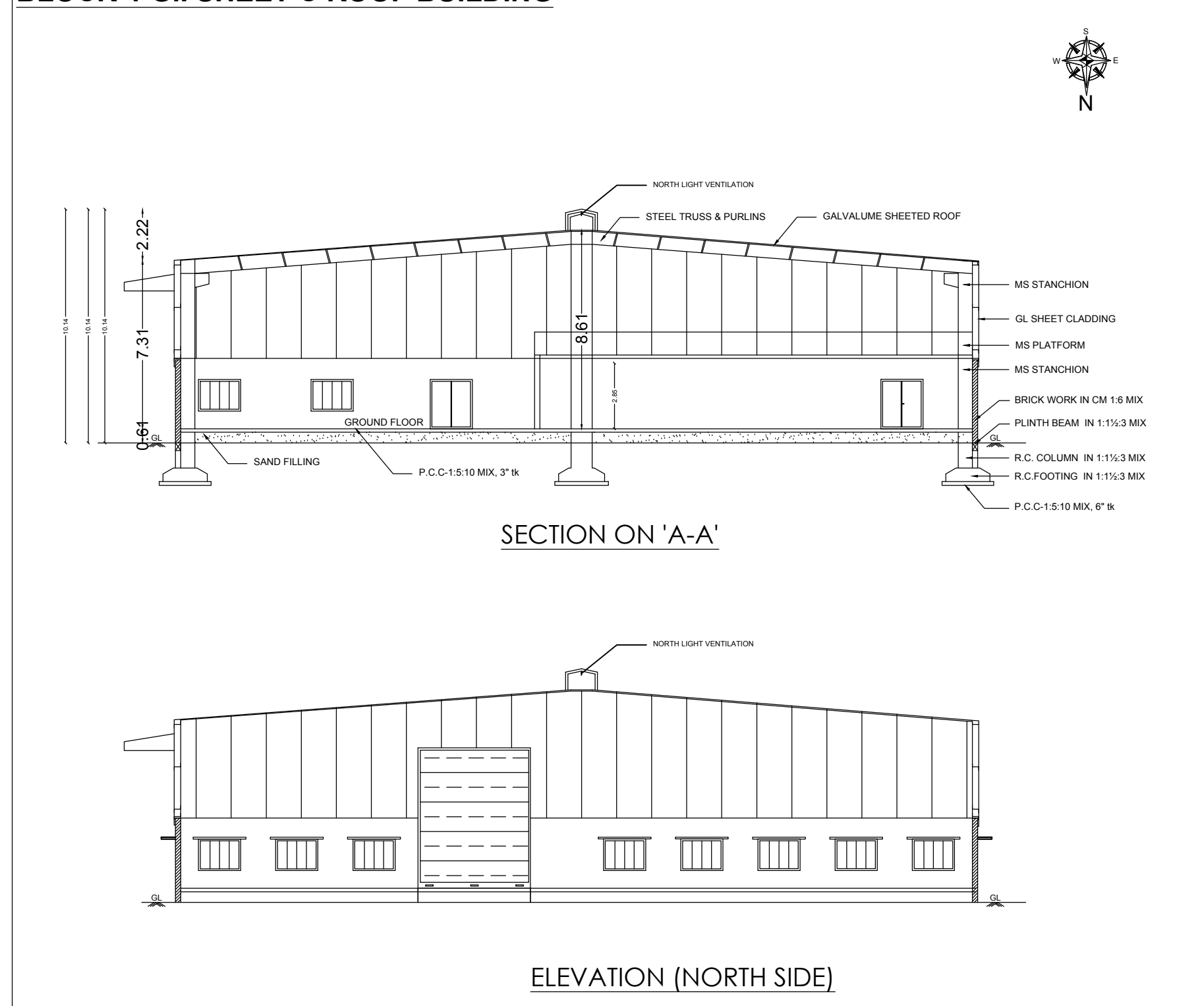
BLOCK-1 G.I. SHEET C ROOF BUILDING
