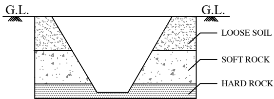
TRIAL PIT
