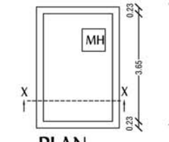
PLAN DETAILS OF U.G. SUMP RAIN WATER COLLECTION SUMP
