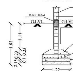
FOUNDATION DETAIL
