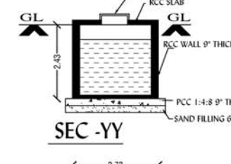
SEC -YY
