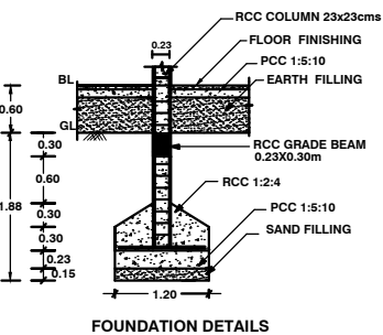
FOUNDATION DETAILS
