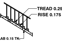
STAIR CASE DETAILS
