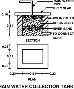
RAIN WATER COLLECTION TANK
