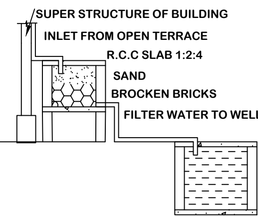
RAINWATER HARVESTING
