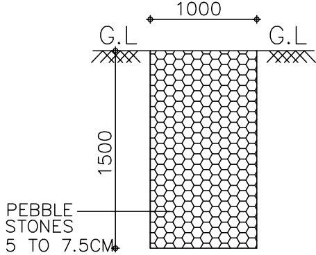
SECTION OF PEBBLE TRENCH SCALE : 1" = 100
