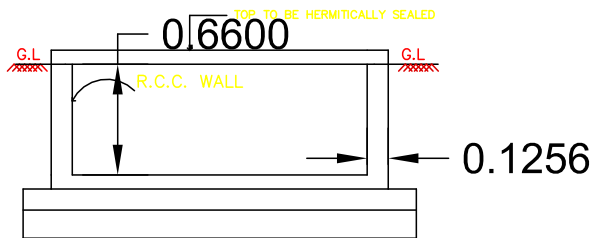
RWH SECTION (SAMPLE) RWH_CAPACITY_L = 2000LTRS
