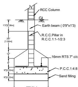
FOUNDATION DETAILS
