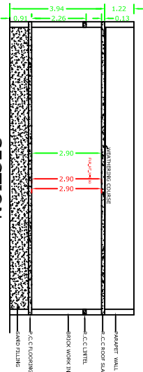
SECTION
