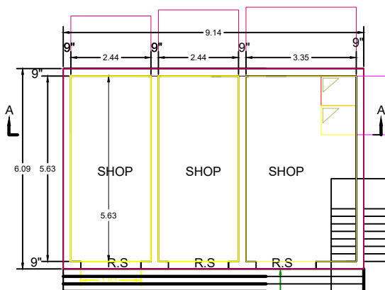
G.F. PLAN
