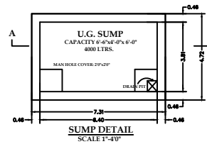
SUMP DETAIL
