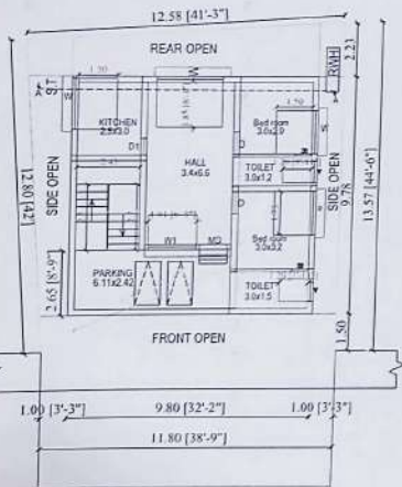
PROPOSED GROUND FLOOR
