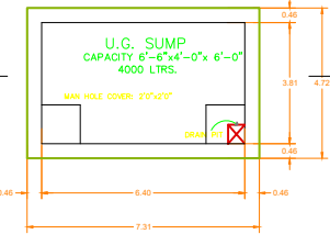
SUMP DETAIL
