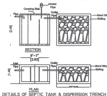
DETAILS OF SEPTIC TANK & DISPERSION TRENCH
