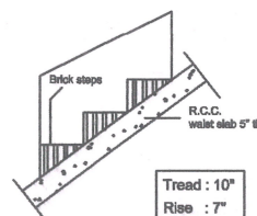
STAIRCASE DETAILS-nts
