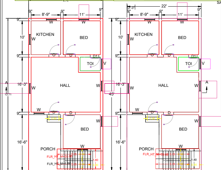
G.F. PLAN
