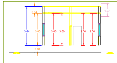
DWARF WALL SECTION NOT TO SCALE
