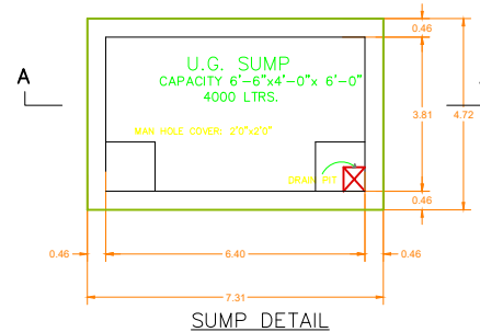
SUMP DETAIL
