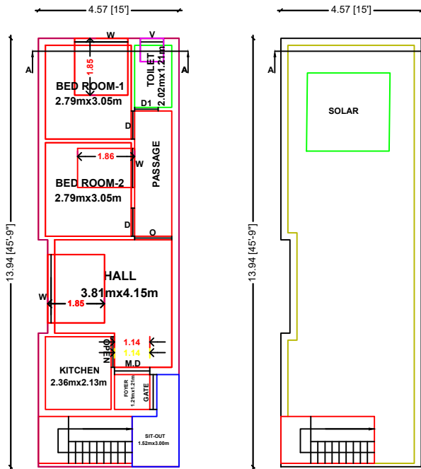
GROUND FLOOR PLAN TERRACE FLOOR PLAN
