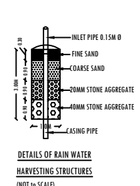
DETAILS OF RAIN WATER HARVESTING STRUCTURES
