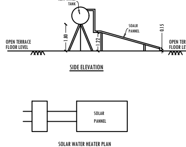
SOLAR WATER HEATER PLAN
