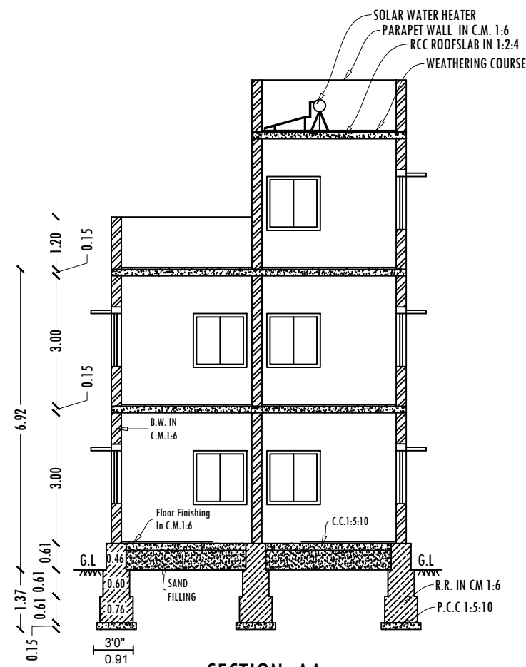
SECTION -AA
