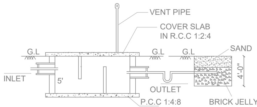
SECTION-AB
