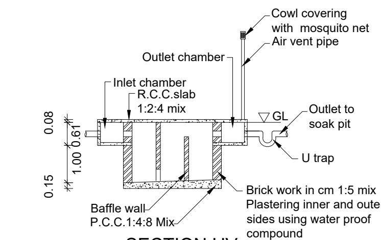
SECTION UV
