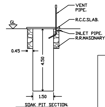
SOAK PIT SECTION.
