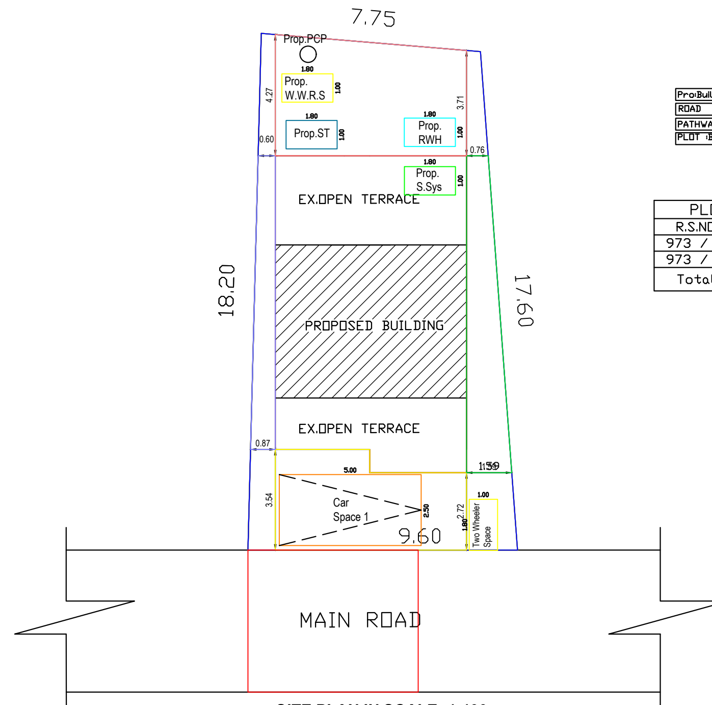
SITE PLAN IN SCALE -1:100 ALL DIMENSIONS ARE IN MTR.
