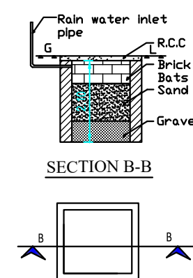
RAIN WATER HARVESTING PIT
