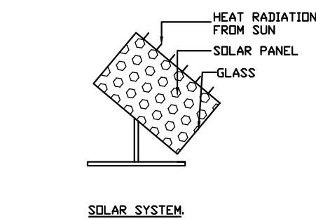
SOLAR SYSTEM.
