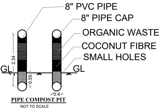
PIPE COMPOST PIT NOT TO SCALE
