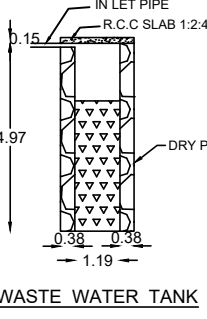
WASTE WATER TANK
