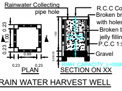
RAIN WATER HARVEST WELL
