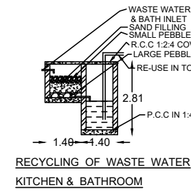
RECYCLING OF WASTE WATER KITCHEN & BATHROOM
